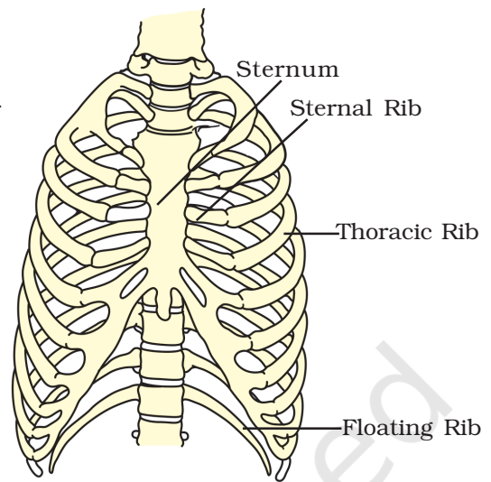
Fig. 33.4 Rib cage and sternum
