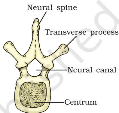
Fig. 33.3 A typical vertebra
